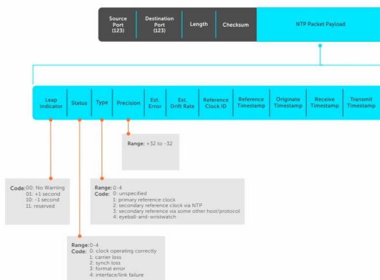
Figure 116. NTP Fields
